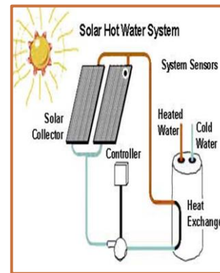
Hot Water Collector
